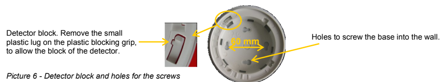
Picture 6 - Detector block and holes for the screws
