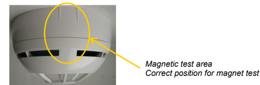
Picture 8 - Magnetic test area
